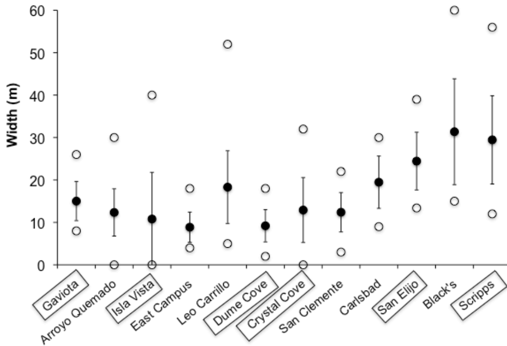
Figure 5 Mean (•)(± one standard deviation) and maximum (o) and minimum (o) values of widths of the active intertidal zone (damp and saturated sand, swash zones) observed for the study beaches in monthly surveys from December 2011 to November 2013. Beaches are listed from north to south. Names of sites located in MPAs are in boxes.
