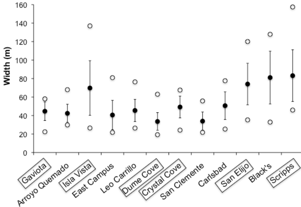
Figure 5 Mean (•)(± one standard deviation) and maximum (o) and minimum (o) values of widths of the active intertidal zone (damp and saturated sand, swash zones) observed for the study beaches in monthly surveys from December 2011 to November 2013. Beaches are listed from north to south. Names of sites located in MPAs are in boxes.
