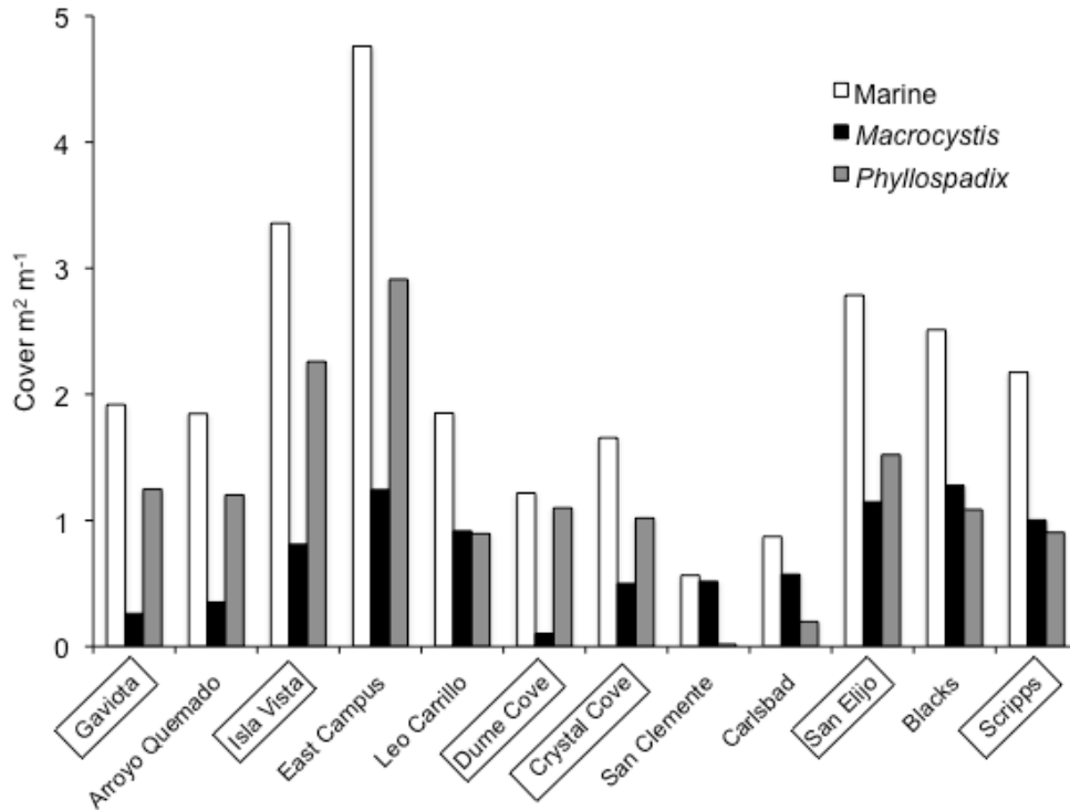
Figure 23. Mean values of cover of marine macrophyte wrack (total marine, Macrocytistis pyrifer and Phyllospadix spp.) expressed as mean cover m 2 m -1 , for monthly surveys of the 12 study beaches from December 2011 to November 2013 (n = 24). Beaches are listed from north to south. Names of sites located in MPAs are in boxes.
