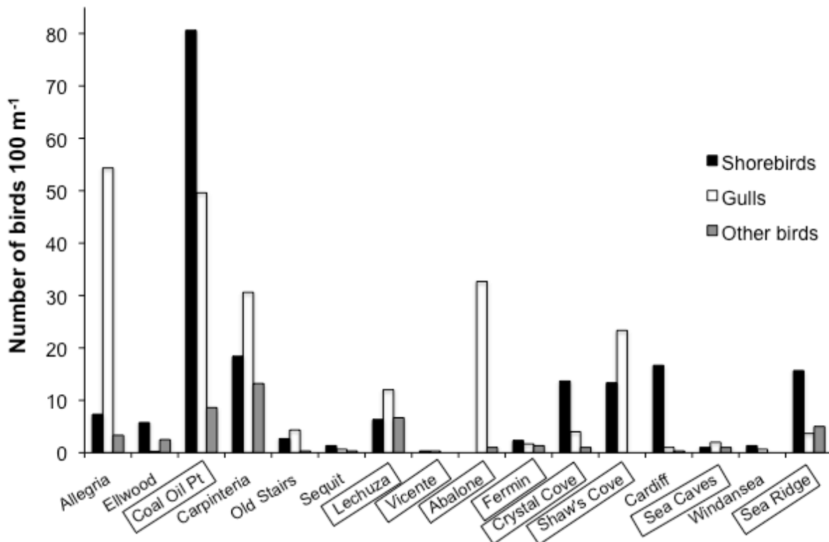
Figure 56 Mean numbers of shorebirds, gulls and other birds observed in surveys of 100 meter rocky intertidal shoreline segments at 16 SC mainland sites between December 2013 and February 2014. Sites are listed from north to south. Names of sites located in MPAs are in boxes
