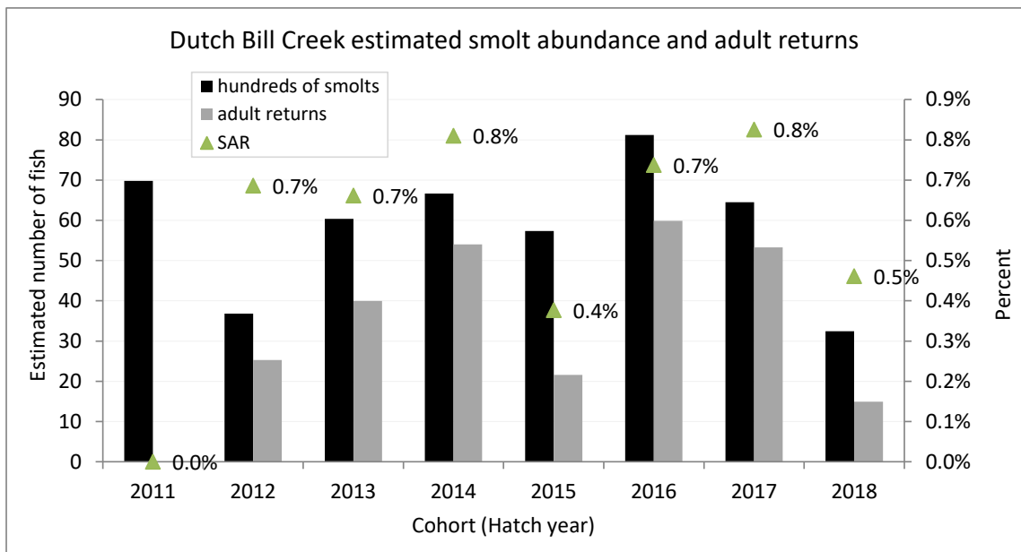
Figure 18. Estimated coho salmon smolt abundance, adult returns and smolt to adult return (SAR) ratios in Dutch Bill Creek, cohorts 2011-2018.
