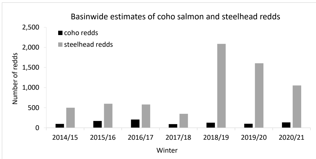
Figure 30. Basinwide estimates of coho salmon and steelhead redds in the Russian River watershed, return winters 2014/15 through 2020/21. Note that prior to winter 2018/19, steelhead redd abundance was only estimated for CMP reaches that also contained coho salmon habitat, while abundance from 2018/19 forward was estimated for all steelhead reaches within the CMP sample frame.
