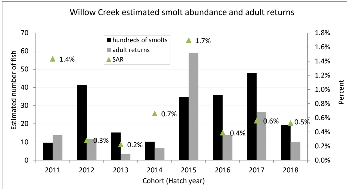
Figure 17. Estimated coho salmon smolt abundance, adult returns and smolt to adult return (SAR) ratios in Willow Creek, cohorts 2011-2018. Note that estimates are based on returns to the upper antennas at river km 3.69.
