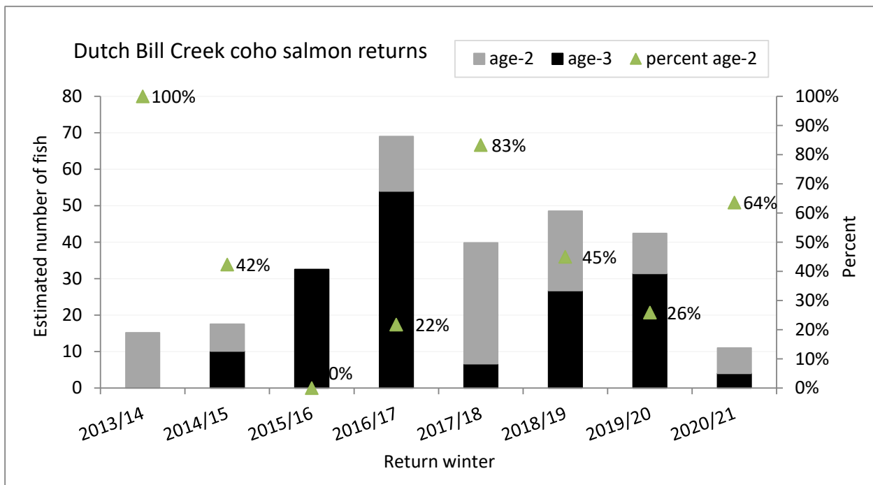
Figure 12. Estimated annual Dutch Bill Creek adult hatchery coho salmon returns by age, return seasons 2013/14 – 2020/21.
