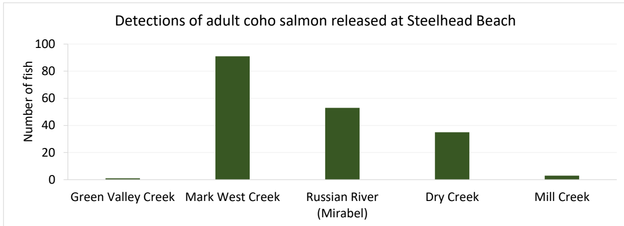
Figure 21. Detections of PIT-tagged adult coho salmon released at Steelhead Beach on January 7, 2021. Note that some individuals were detected at multiple sites.
