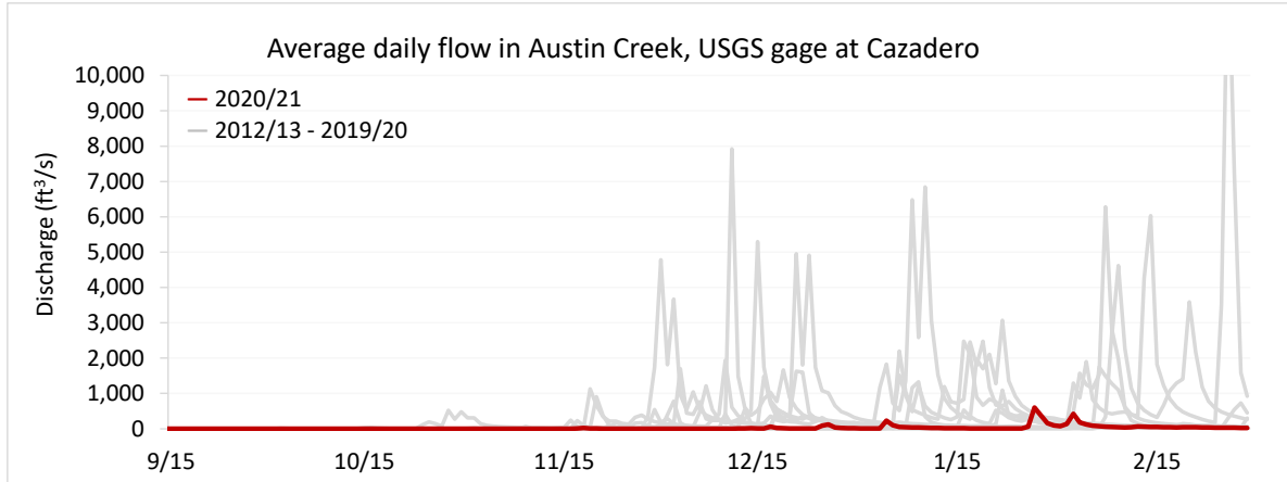
Figure 4. Winter 2020/21 streamflow in Austin Creek as compared to streamflow during the previous eight winters. Data was downloaded from the USGS website .
