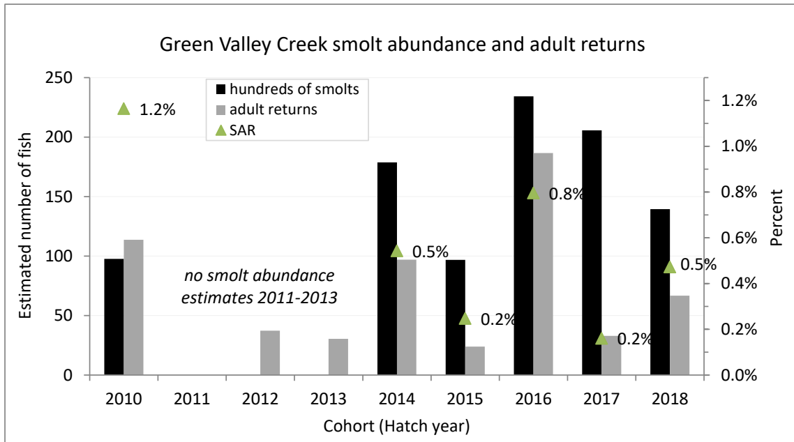
Figure 19. Estimated coho salmon smolt abundance, adult returns and smolt to adult return (SAR) ratios in Green Valley Creek, cohorts 2010-2018. Note that adult release fish returning to Green Valley Creek were excluded from SAR calculations.
