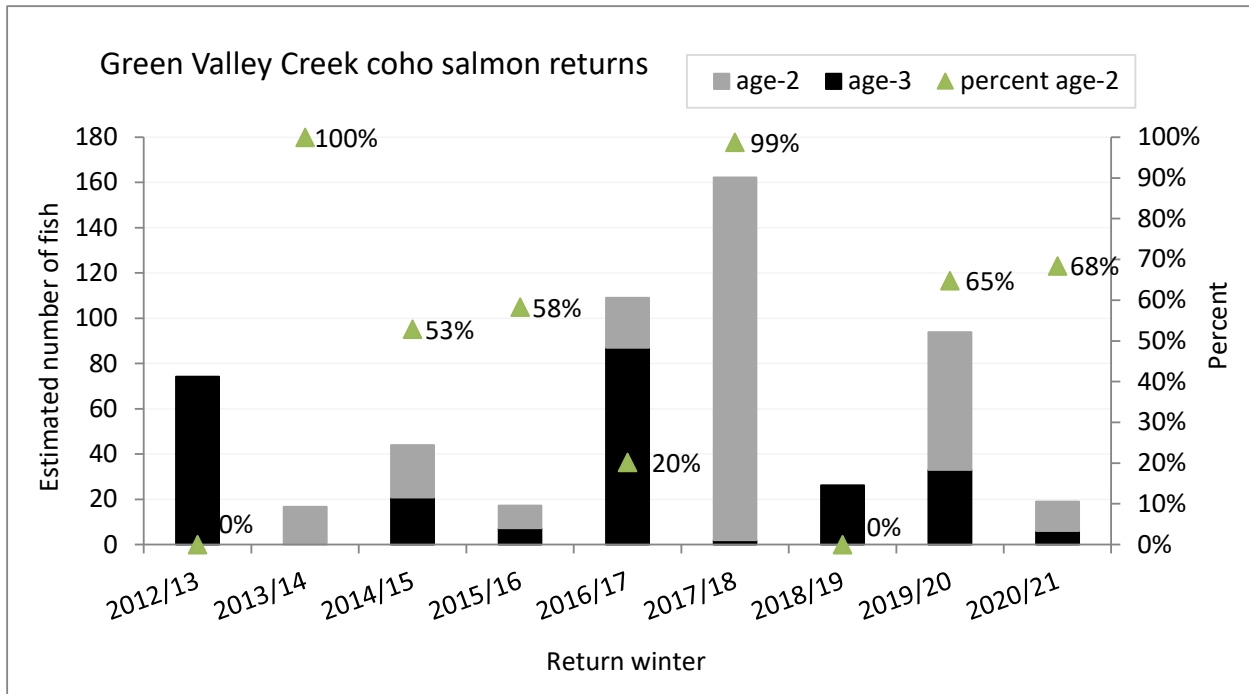
Figure 13. Estimated annual Green Valley Creek adult hatchery coho salmon returns by age, return seasons 2012/13 – 2020/21.
