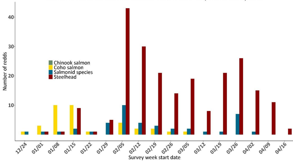
Figure 27. Number of new salmonid redds observed each week in Russian River Coastal Monitoring Program survey streams, winter 2020/21.
