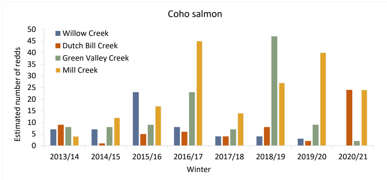
Figure 28. Estimated coho salmon redds in Broodstock Program monitoring tributaries, return winters 2013/14 through 2020/21.
