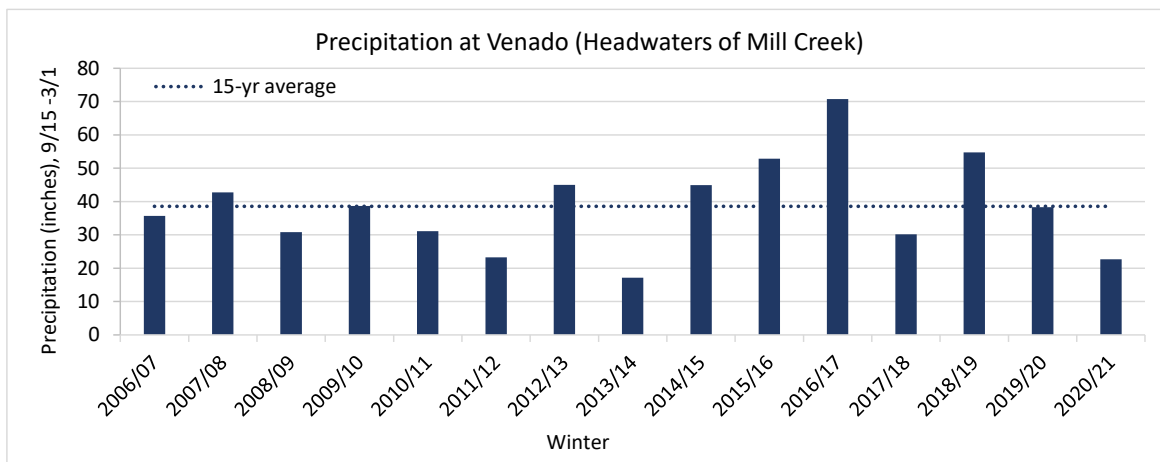
Figure 3. Precipitation at Venado gage near Mill Creek headwaters. Data was downloaded from the NOAA website .
