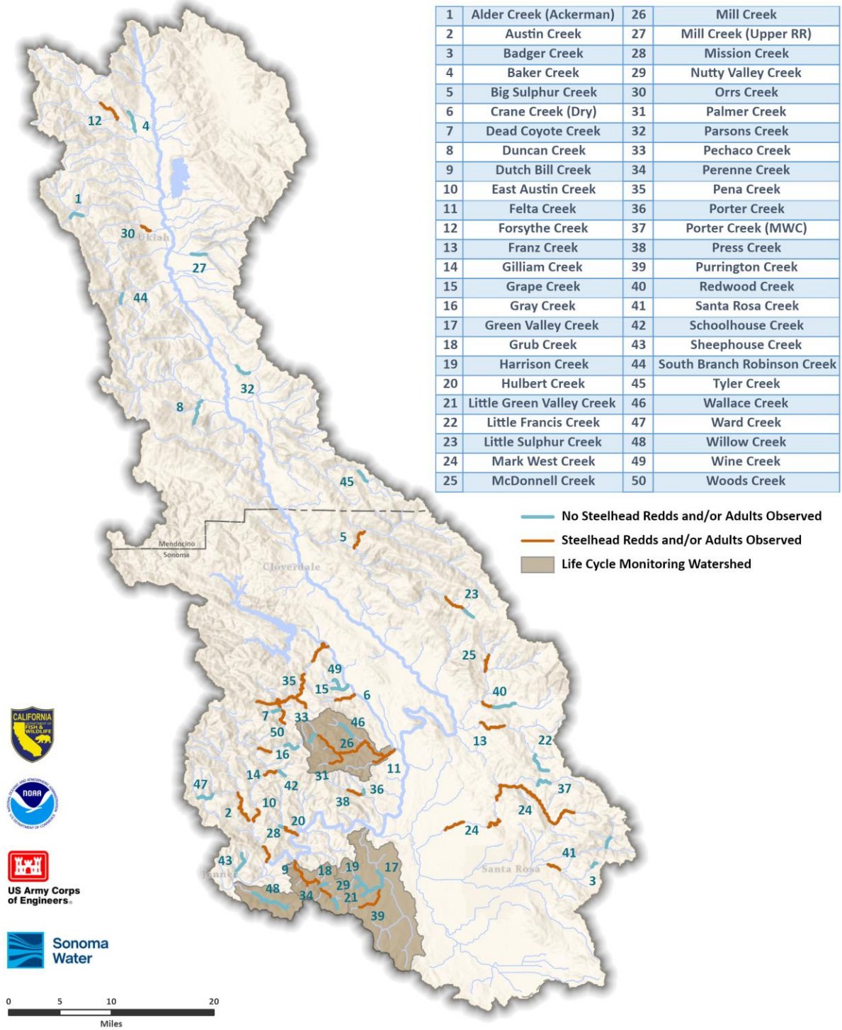
Figure 26. Spawner survey reaches where steelhead redds and/or live steelhead adults were observed, winter 2020/21.
