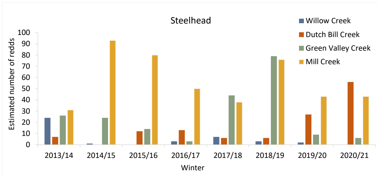
Figure 29. Estimated steelhead redds in Broodstock Program monitoring tributaries, return winters 2013/14 – 2020/21.
